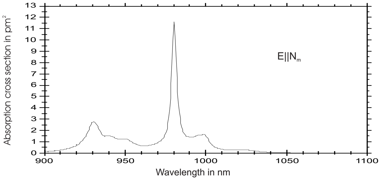
Emission and absorption spectra of KYbW (100at.% Yb:KYW, stoichiometric KYbW)
